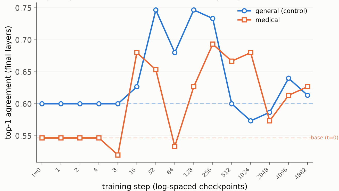
Top-1 agreement is noise-dominated at 15 prompts / arm
