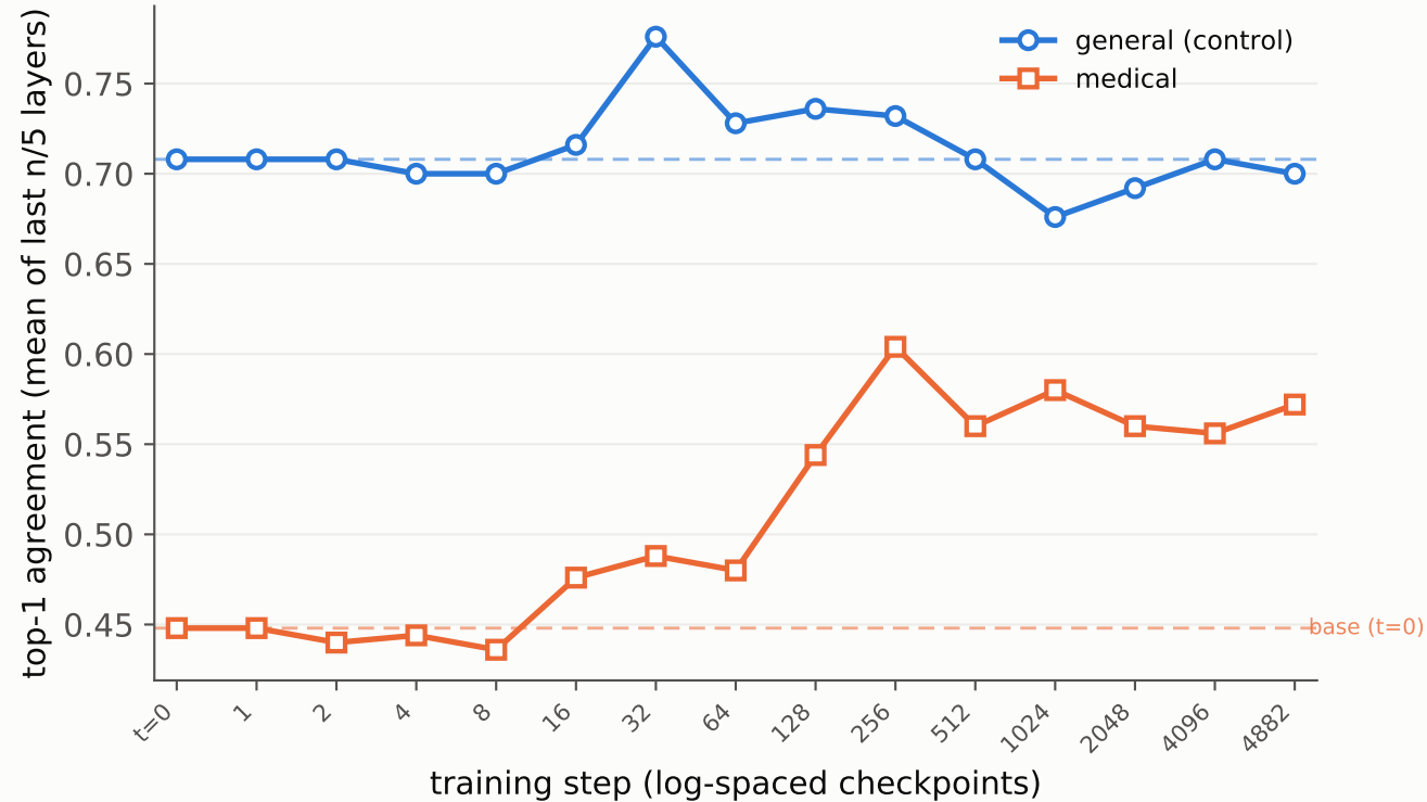
Gemma-3-1b-it — top-1 agreement vs. the untuned base
