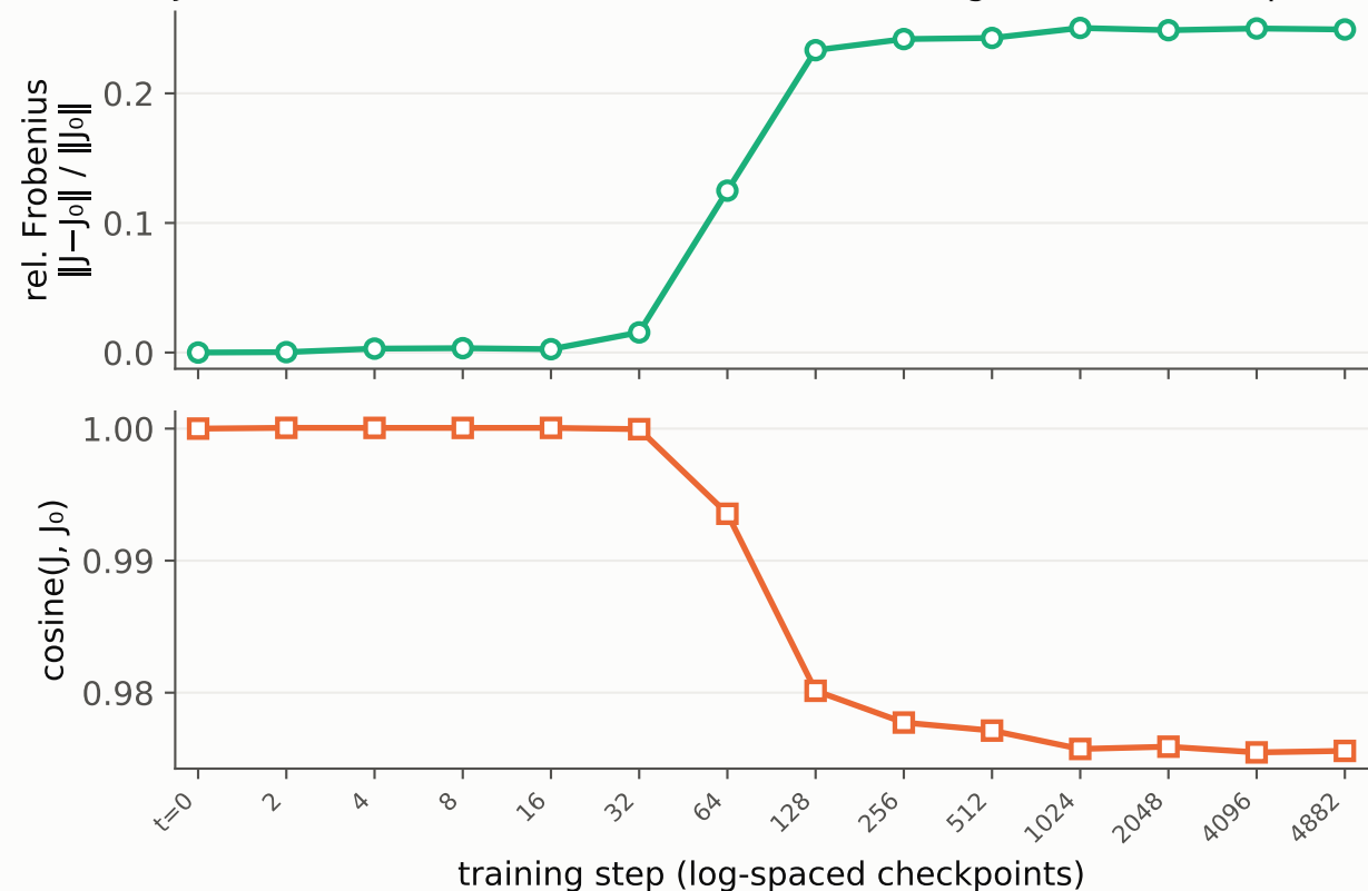
Jacobian drift from the base lens — fast reorganization, then plateau
