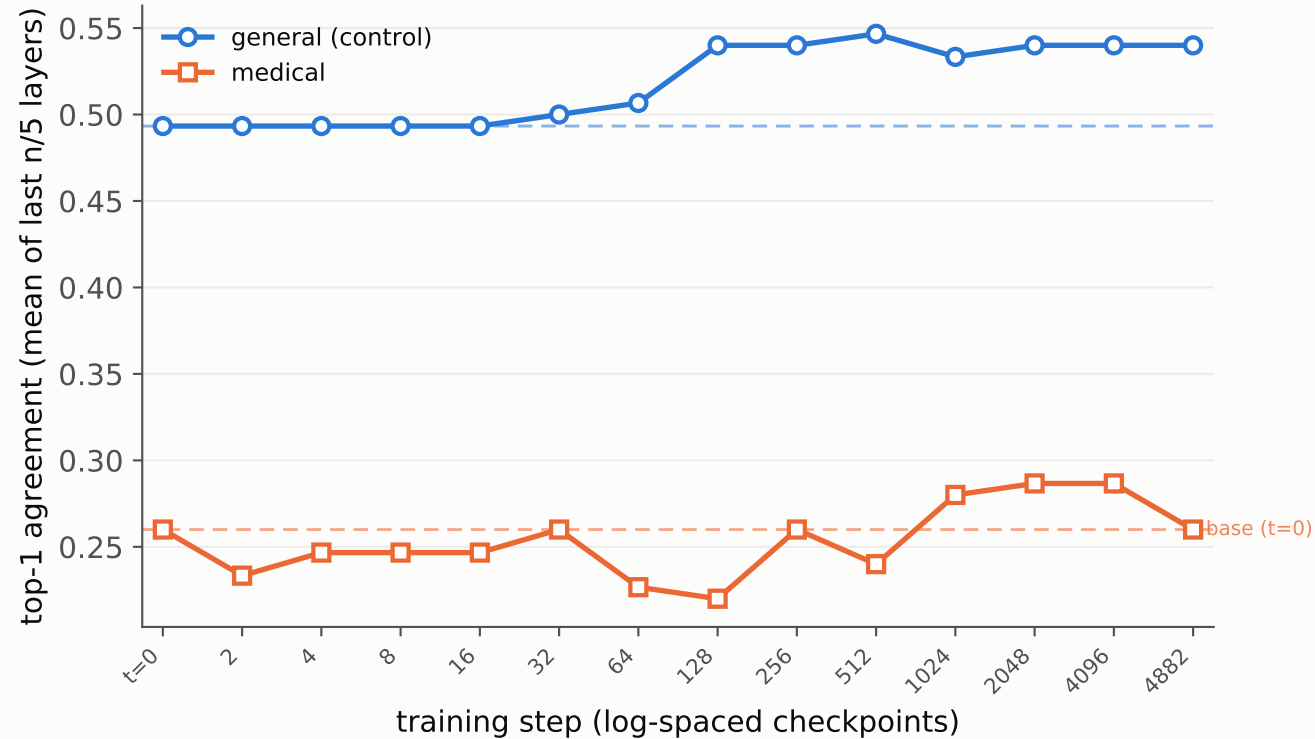
Gemma-3-270m-it — top-1 agreement vs. the untuned base
