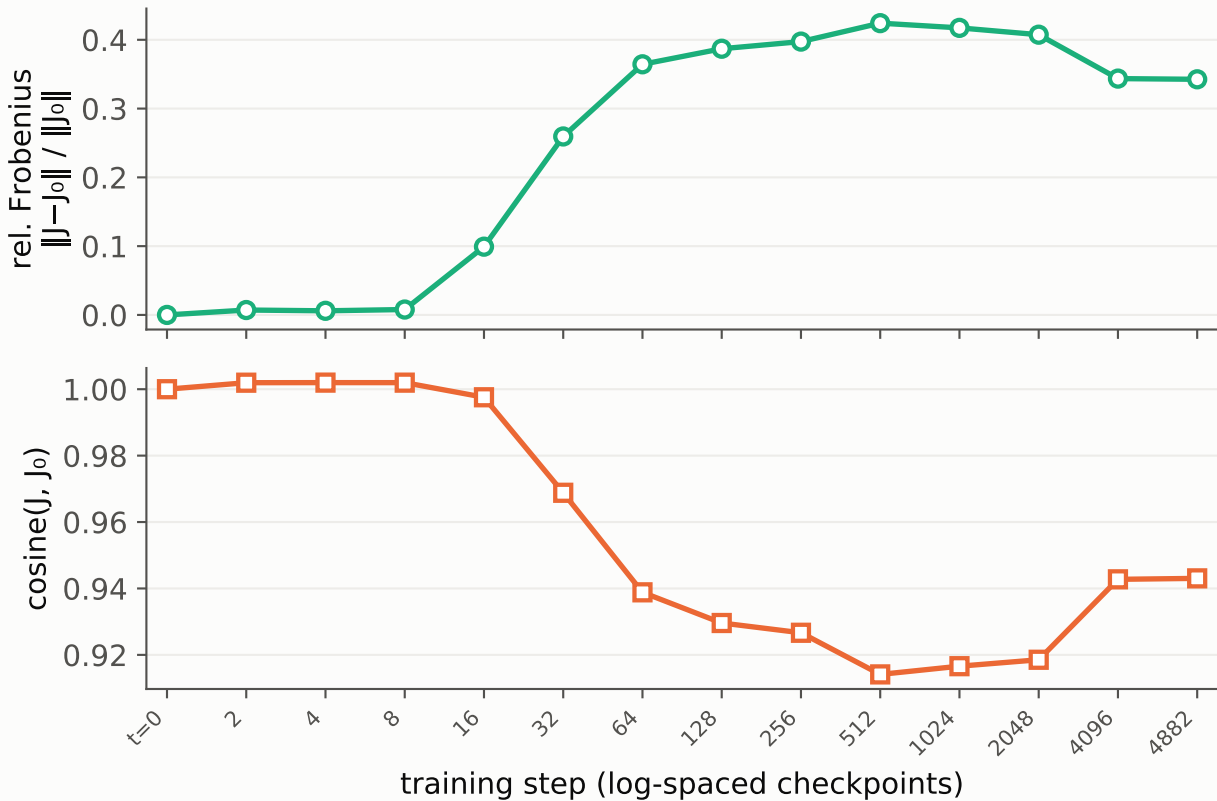
gemma-3-4b-it — Jacobian drift from the base lens
