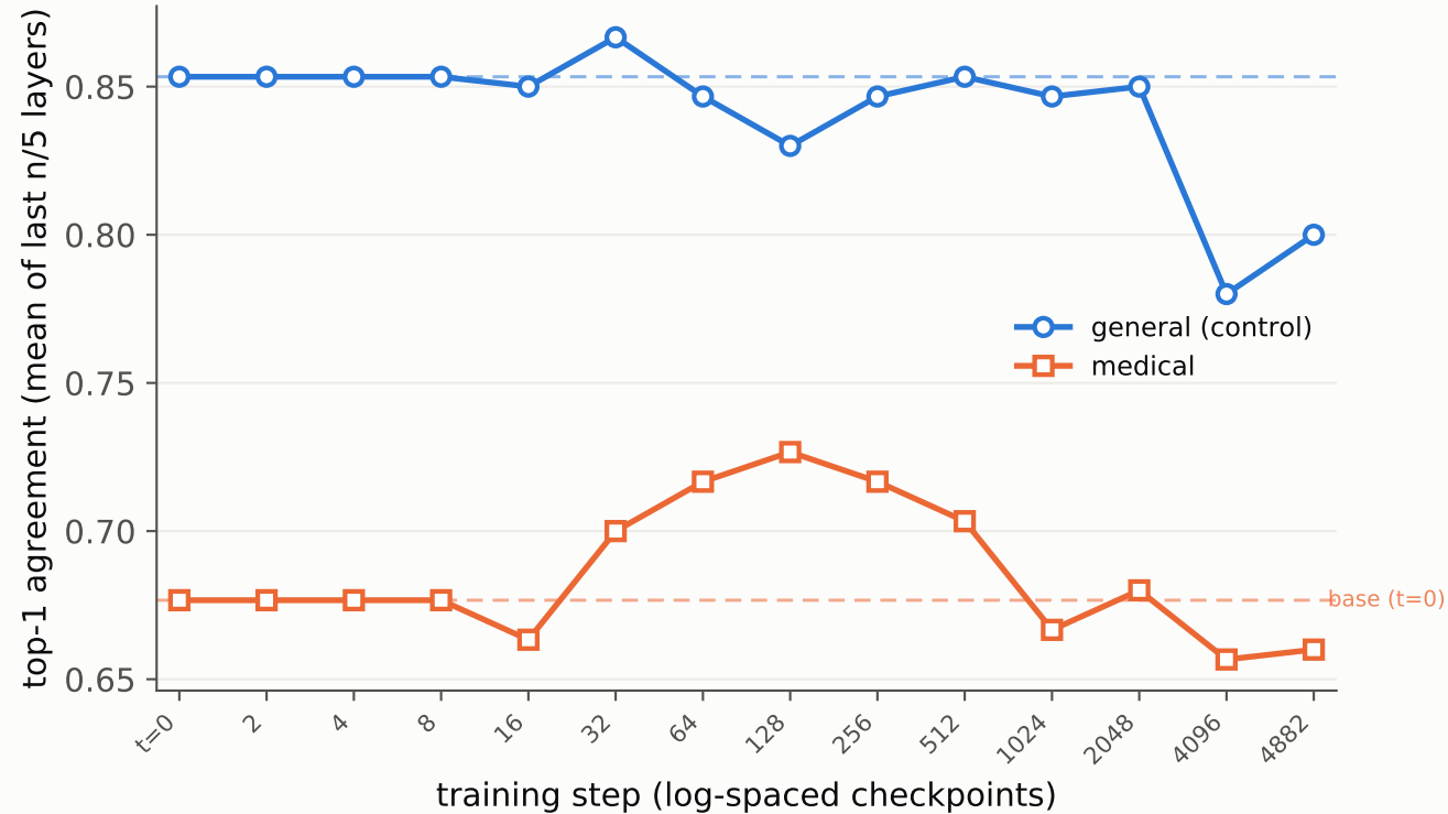
gemma-3-4b-it — top-1 agreement vs. the untuned base
