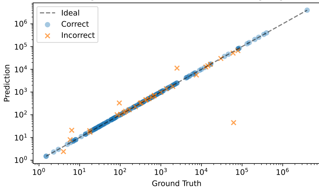
Strong PoT: Prediction vs Ground Truth (Log-Log)
