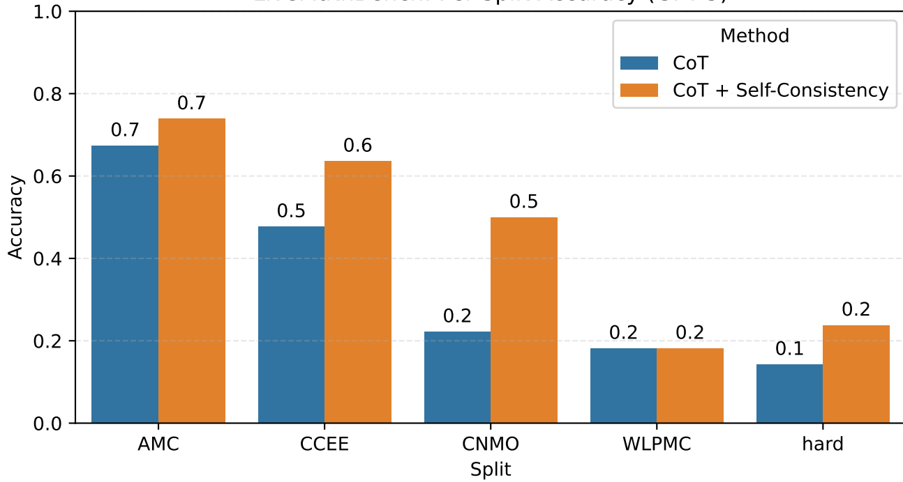
LiveMathBench: Per-Split Accuracy (GPT-5)
