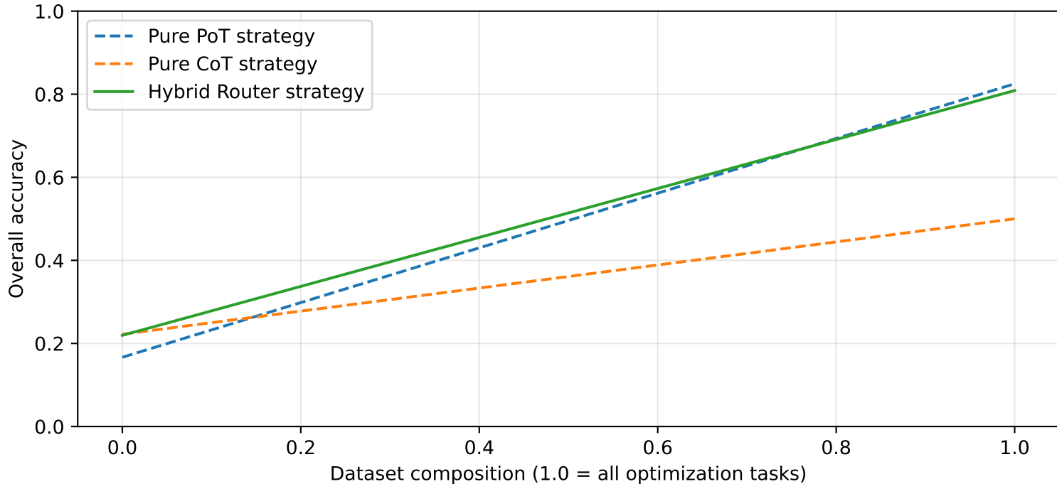
Router Performance vs Task Mix
