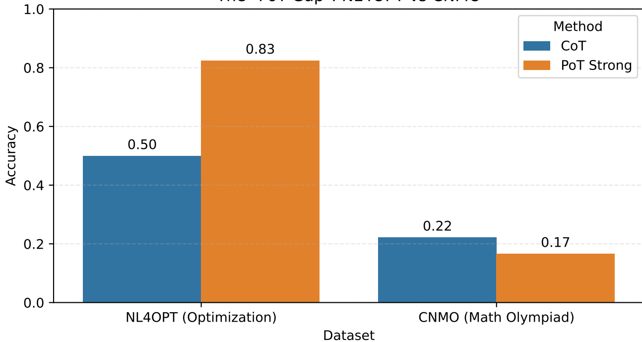
The "PoT Gap": NL4OPT vs CNMO
