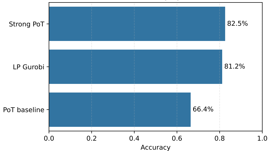
NL4OPT: Accuracy by Method
