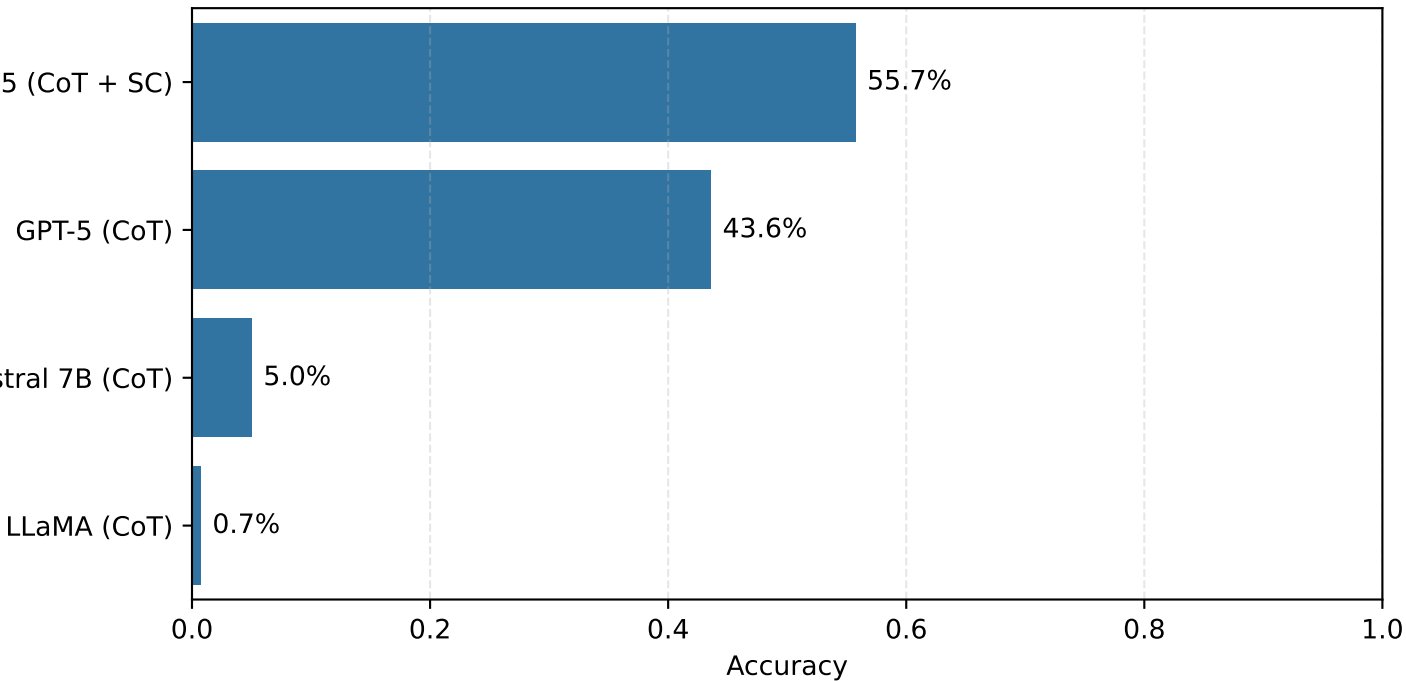
LiveMathBench: Overall Model Leaderboard
