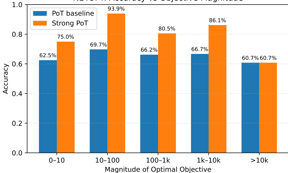
NL4OPT: Accuracy vs Objective Magnitude
