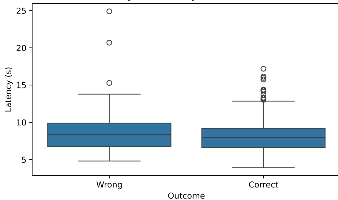
Strong PoT: Latency vs Correctness
