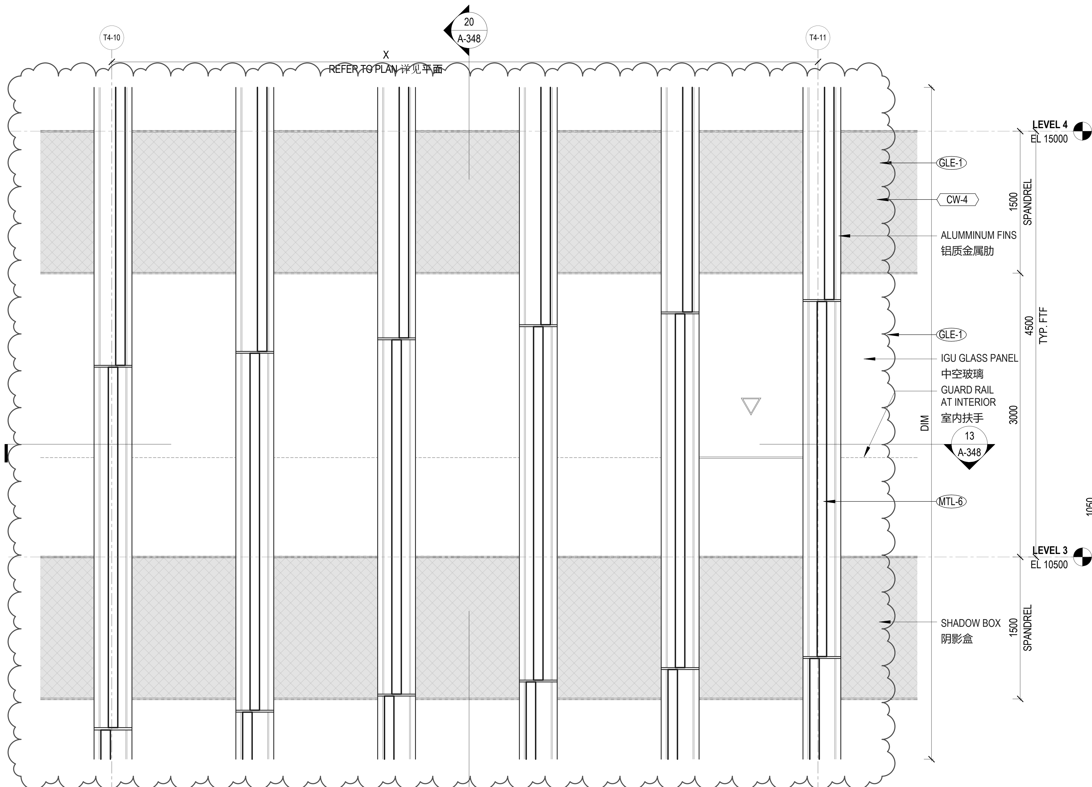
TYPICAL T4 (CW-4) - ELEVATION
