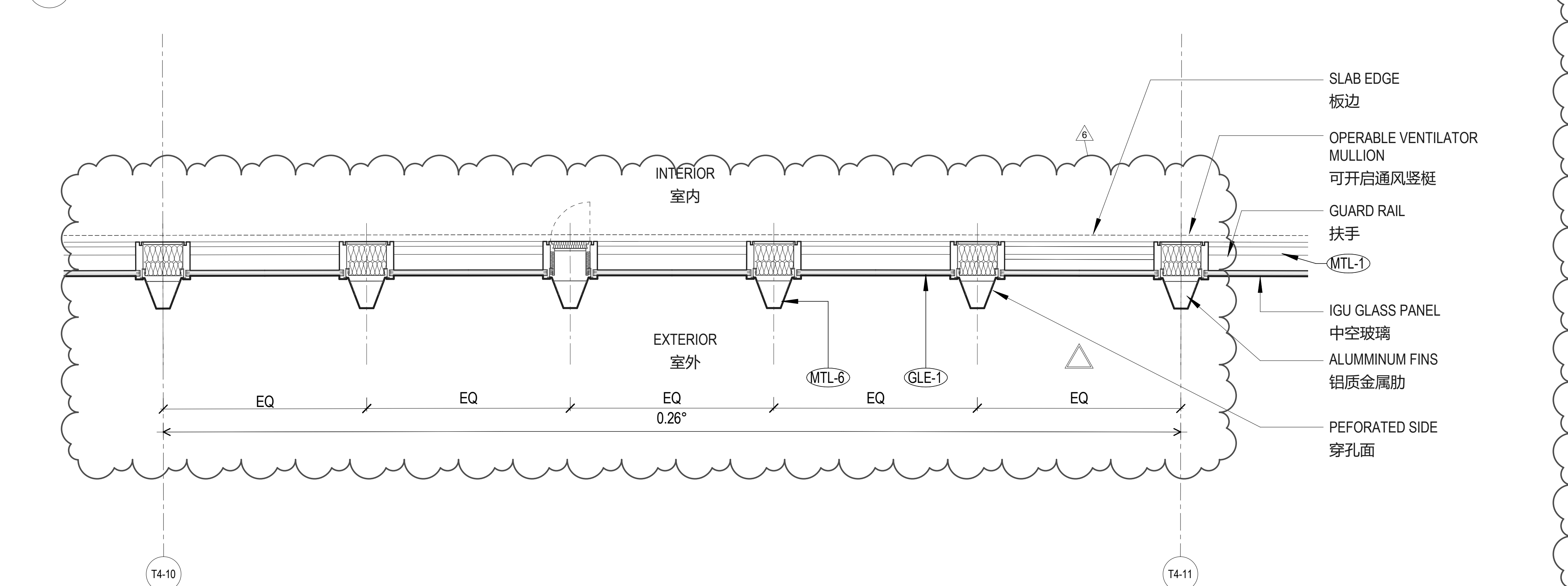
TYPICAL T4 (CW-4) - PLAN
