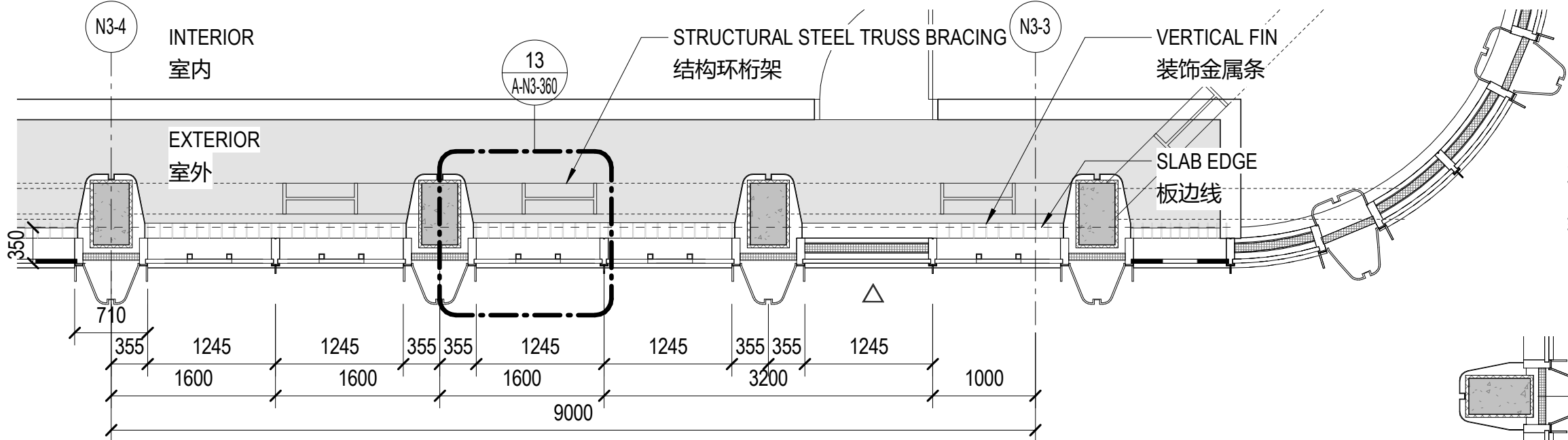
CW-1 ENLARGED PLAN - AT REFUGE FL. CW-1 放大平面-避难层
