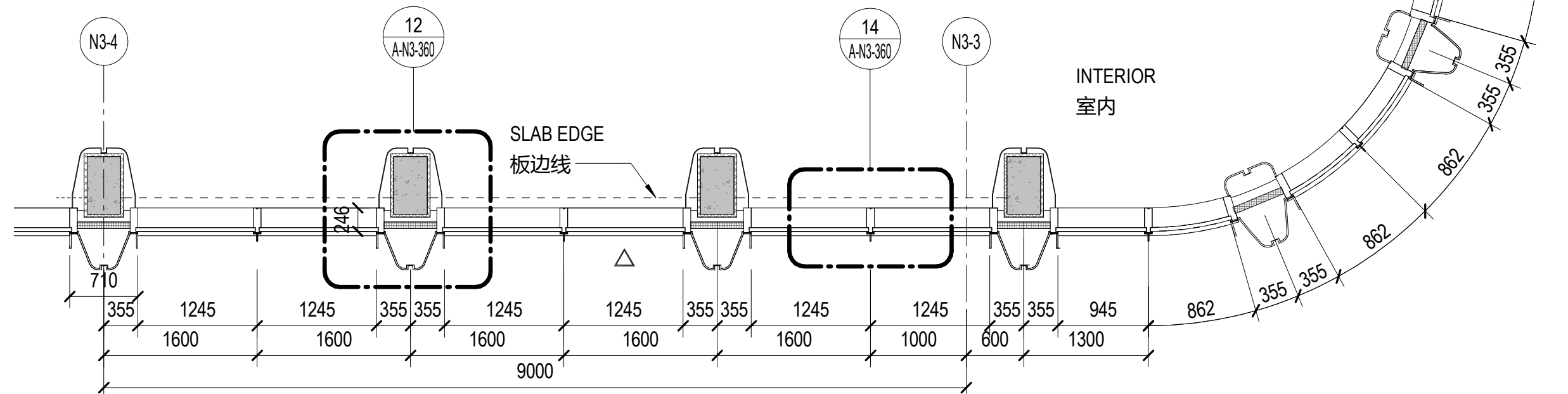
CW-1 ENLARGED PLAN - TYP. CW-1 放大平面-标准层
