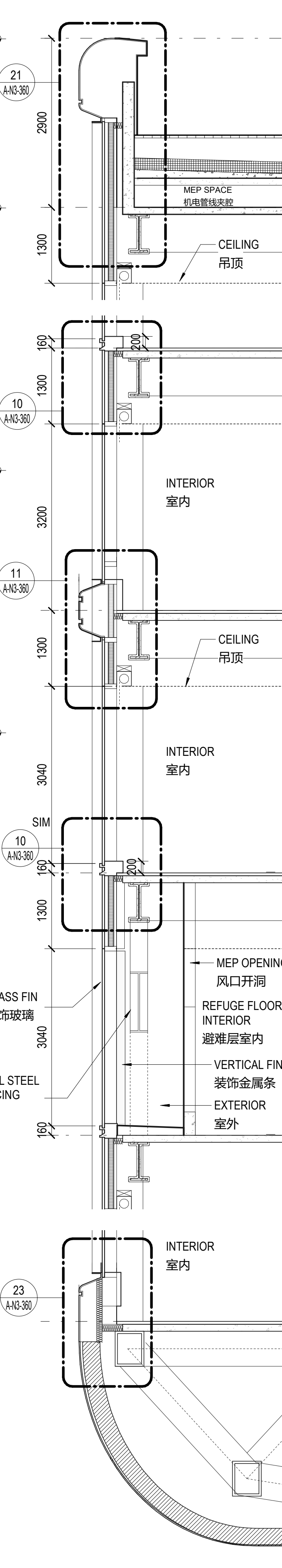
CW-1 ENLARGED SECTION - TYP. CW-1放大剖面-标准层
