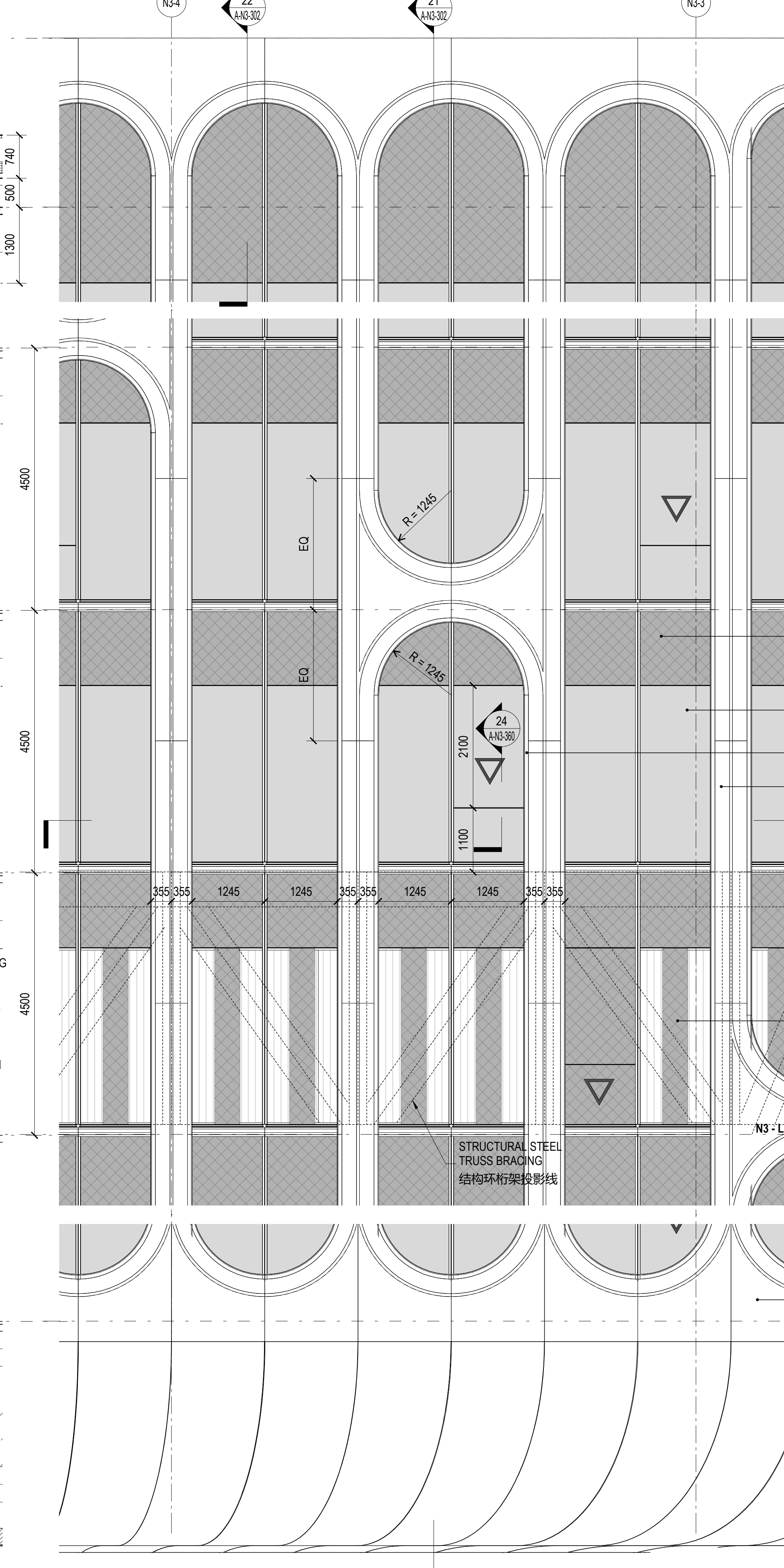
CW-1 ENLARGED ELEVATION CW-1放大立面-标准段
