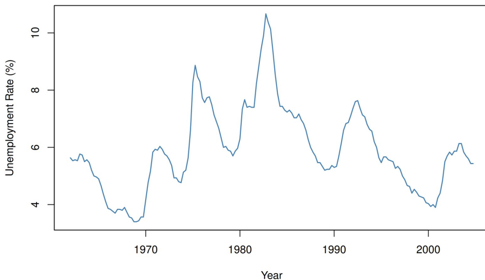
Figure 7: U.S. unemployment rate, uratet, 1962:Q3-2004:Q4.
