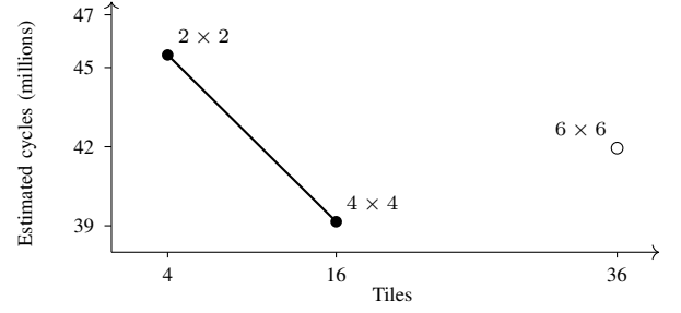
Fig. 2. Cycle/tile frontier from the archived run. Filled points are nondominated; 6 \times 6 is dominated by 4 \times 4 .
