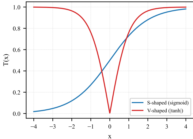
Transfer functions
