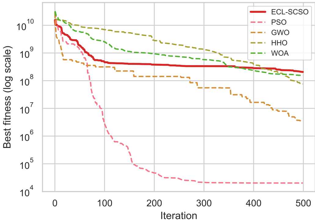
CEC2017_F12
