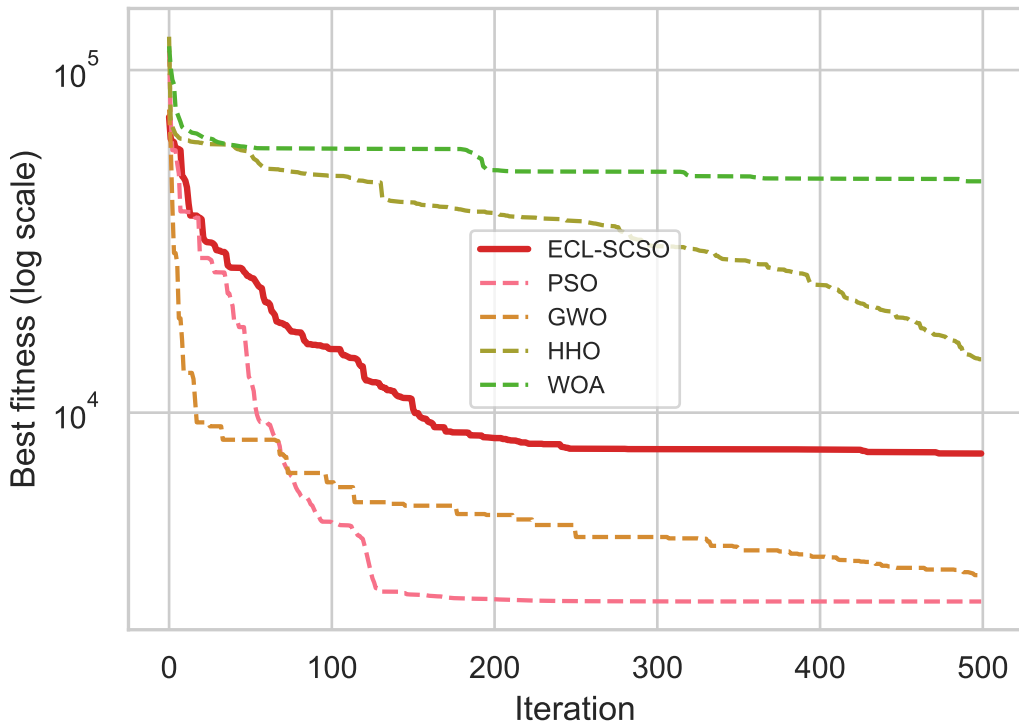
CEC2017_F20
