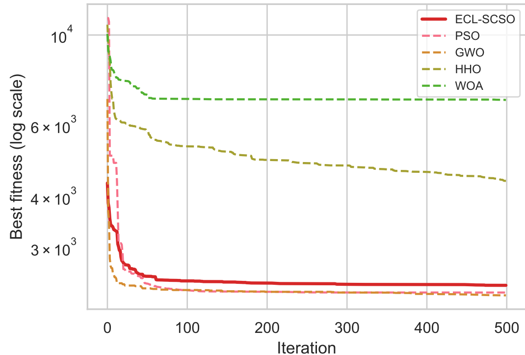
CEC2017_F21
