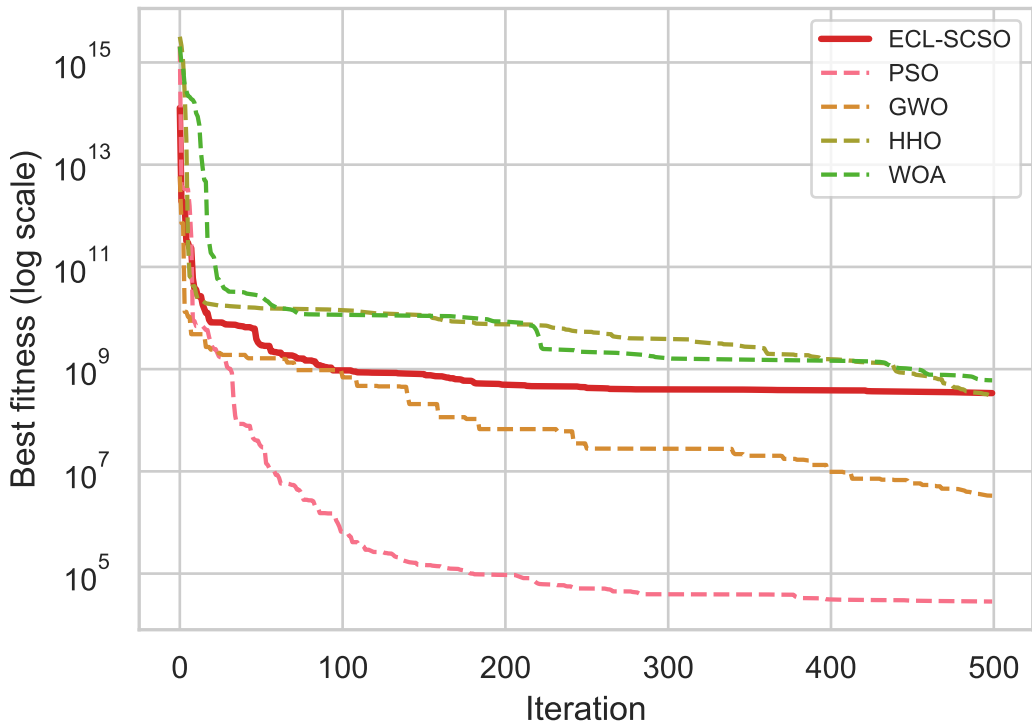
CEC2017_F29
