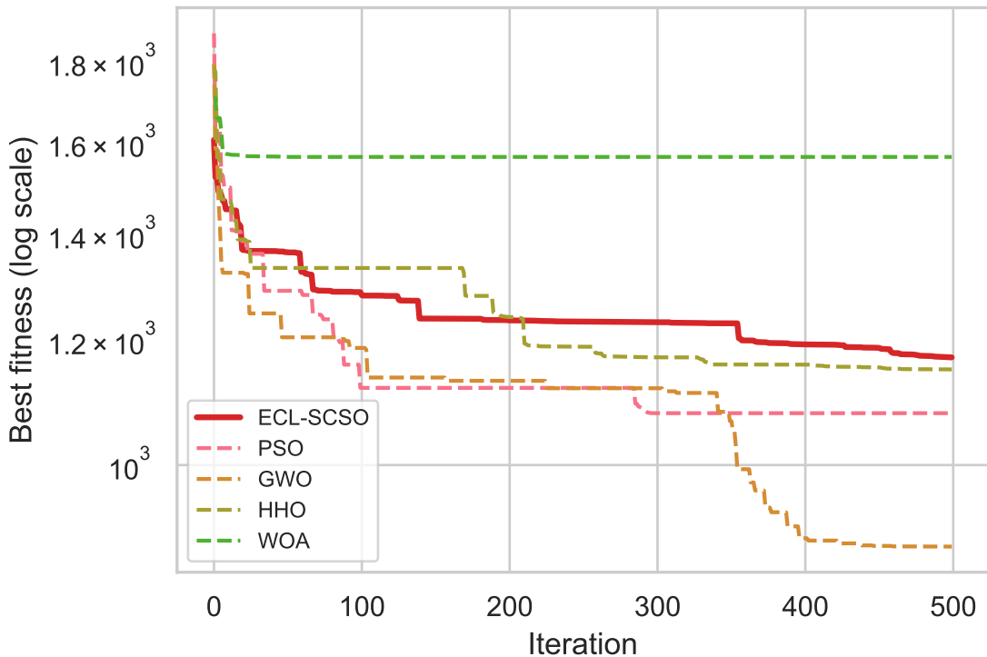
CEC2017_F7
