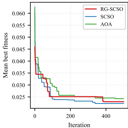
Zoo
