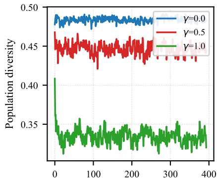
Zoo
