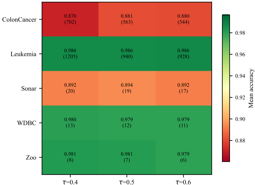
Threshold sensitivity: accuracy (mean #features)
