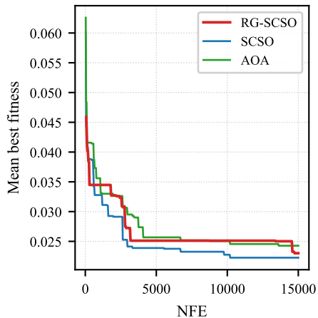
Zoo
