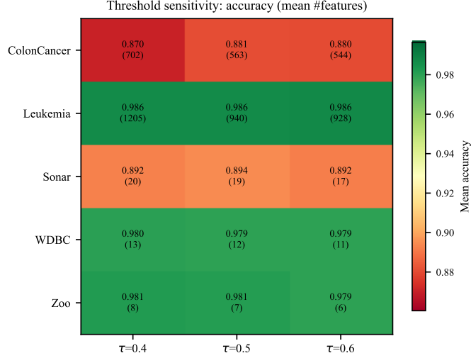
Figure 6: Mean held-out accuracy (color) and mean number of selected features (in parentheses) across the three preferred-bit thresholds tested ( \tau \in \{0.4, 0.5, 0.6\} ), one row per dataset. Accuracy is essentially flat across thresholds on every dataset (largest swing 0.011, ColonCancer \tau=0.4 vs. \tau=0.5 ), while the selected-feature count falls monotonically as \tau increases on all five datasets, confirming \tau = 0.5 is not a fragile choice.
