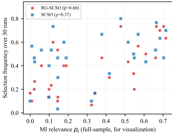
(a) WDBC: relevance vs. selection
