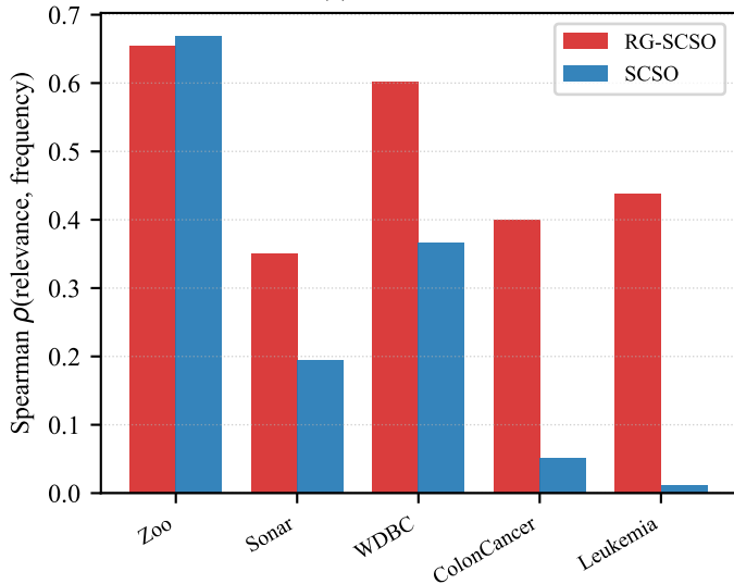
(b) Across datasets
