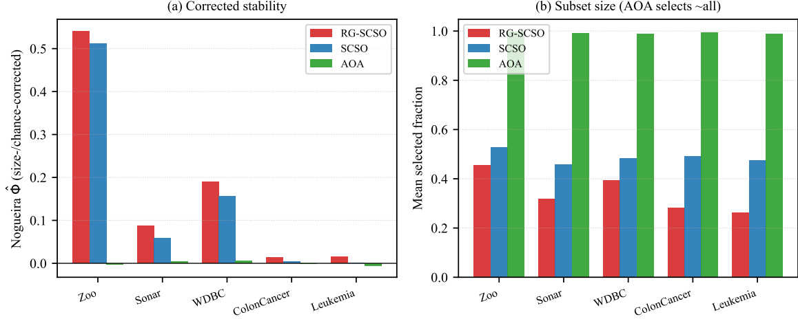
Figure 9: Feature-subset stability across the five representative datasets, 30 runs each. (a) Size- and chance-corrected Nogueira \hat{\Phi} : RG-SCSO exhibited more size-corrected run-to-run stability than the baseline SCSO on every evaluated dataset, while AOA sits at \hat{\Phi} \approx 0 (no better than chance). (b) Mean selected fraction, explaining why an uncorrected metric misleads: AOA selects \approx 98 – 99\% of all features, so its subsets trivially overlap, whereas RG-SCSO selects the fewest. Raw pairwise Jaccard (confounded by this size imbalance) is provided only as a Supplementary diagnostic.
