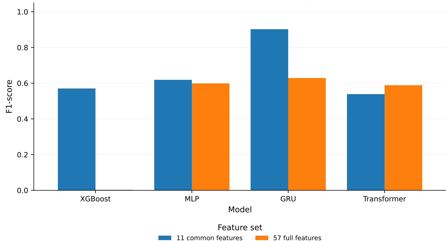
LOIC-HTTP Holdout: Feature-Set Comparison
