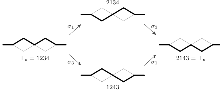
Figure 1: The four runs over a degree-two chain e = \vee[2, 2] . Each panel draws the two blocks of e as squares and the run as the monotone path by which it traverses them, the upper route through a block firing its two events in order and the lower route reversing them. The poset \mathcal{R}(e) is the diamond, and the two routes from \perp_e to \top_e are \text{src}(e) = \sigma_1\sigma_3 and \text{tgt}(e) = \sigma_3\sigma_1 .
