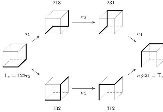
Figure 2: The six runs over a degree-two chain e = \vee[3] . Each panel draws the single block of e as a cube, with the initial vertex of e at the near bottom left and its final vertex at the far top right, and the run as the monotone edge path between them. Here \mathcal{R}(e) is a hexagon, and its two routes are \text{src}(e) = \sigma_1\sigma_2\sigma_1 and \text{tgt}(e) = \sigma_2\sigma_1\sigma_2 .
