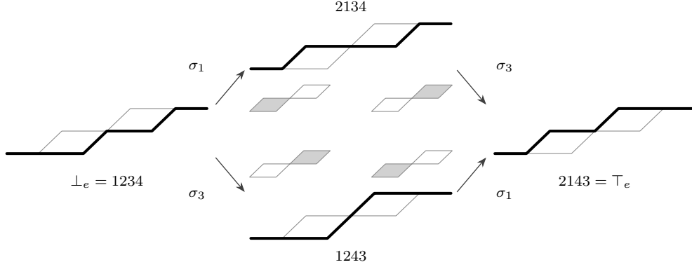
Figure 1: The four runs over a degree-two chain e = \vee[2, 2] . Each panel draws the two blocks of e as squares glued at a vertex, with the edges of the chain before and after them as a tail and a tip, and the run as the monotone edge path it traverses them by. Here \mathcal{R}(e) is a diamond, and its two routes are \text{src}(e) = \sigma_1\sigma_3 and \text{tgt}(e) = \sigma_3\sigma_1 . Each arrow carries a small copy of e with the square it flips shaded: the run is pushed across that square.
