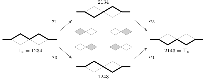
Figure 1: The four runs over the degree-two chain e = \vee[2, 2] , whose two blocks are the events \{1, 2\} and \{3, 4\} , so that \text{cut}(e) = \{1, 3\} . Each panel draws the blocks as squares, with the edges of the chain before and after them as a tail and a tip; the run passes over a square when it fires that block's two events in order and under it when it reverses them. Here \mathcal{R}(e) is a diamond, and its two routes are \text{src}(e) = \sigma_1\sigma_3 and \text{tgt}(e) = \sigma_3\sigma_1 . Each arrow carries a small copy of e with the square it flips shaded.
