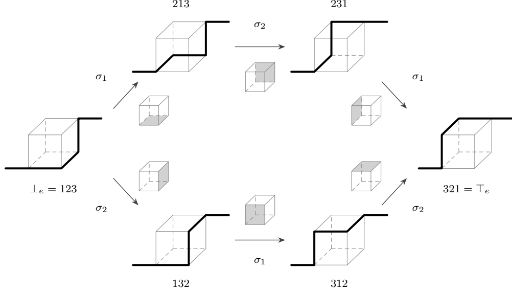
Figure 2: The six runs over the degree-two chain e = \vee[3] , whose single block is the events \{1, 2, 3\} , so that \text{cut}(e) = \{1, 2\} . Each panel draws the block as a cube, with the initial vertex of e at the near bottom left and its final vertex at the far top right, the run as the monotone edge path between them, and the edges of the chain before and after e as a tail and a tip. Here \mathcal{R}(e) is a hexagon, and its two routes are \text{src}(e) = \sigma_1\sigma_2\sigma_1 and \text{tgt}(e) = \sigma_2\sigma_1\sigma_2 . Each arrow carries a small copy of the cube with the square it flips shaded: the run is pushed across that face.
