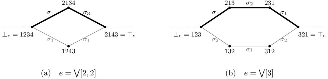
Figure 1: The polygon \mathcal{R}(e) for the two species of degree-two chain (Proposition 4.13). A vertex is the run firing the events of e in the order shown; an edge is the 1-cell it reads as under \gamma (Lemma 7.3). The heavy route is \text{src}(e) and the light one \text{tgt}(e) . The dotted stubs are the rest of \mathcal{R}(d) for a chain d that e refines to, into which the polygon order-embeds (Proposition 4.4).
