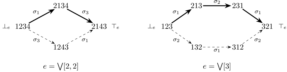
Figure 1: The poset \mathcal{R}(e) for the two species of degree-two chain (Proposition 4.13). A vertex is labelled by the order in which that run fires the events of e , an edge by the 1-cell it reads as under \gamma (Lemma 7.3). The solid chain is \text{src}(e) and the dashed one \text{tgt}(e) .
