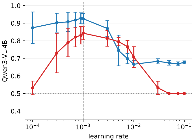
agreement accuracy
