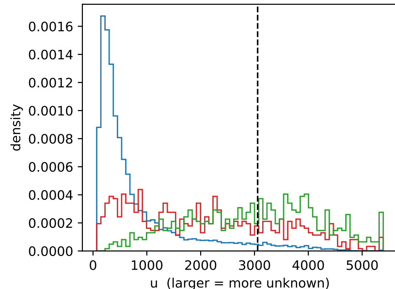
Mahalanobis: min class distance
