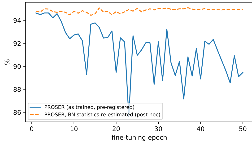
CIFAR-10 validation accuracy (10 known logits)
