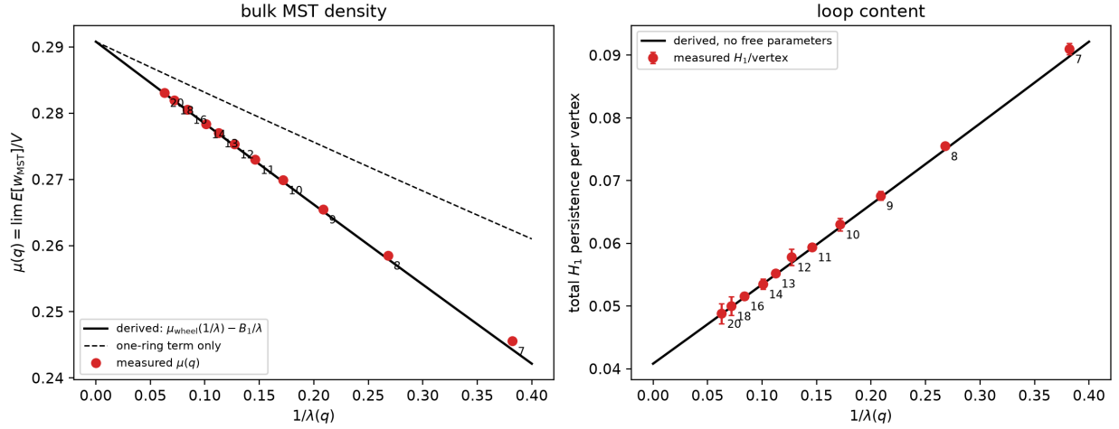
Figure 1: Left: measured \mu(q) against 1/\lambda(q) , with the derived curve (7) (solid) and the one-ring term \mu_{\text{wheel}} alone (dashed). Right: measured total H_1 per vertex with the derived curve (8). Neither curve has a fitted parameter.
