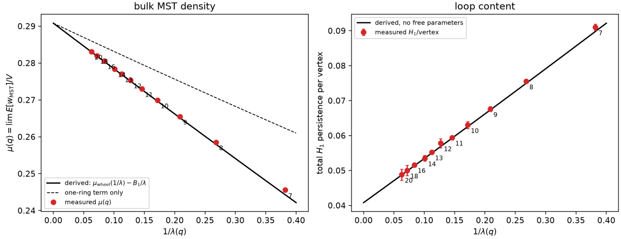
Figure 2: Left: measured \mu(q) against 1/\lambda(q) , with the derived curve (7) (solid) and the one-ring term \mu_{\text{wheel}} alone (dashed). Right: measured total H_1 per vertex with the derived curve (8). Neither curve has a fitted parameter.
