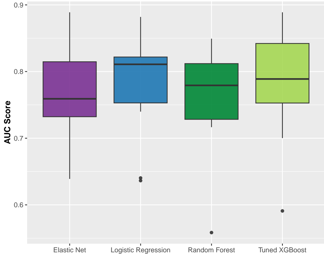
AUC Distribution Across 10-Fold Cross Validation
