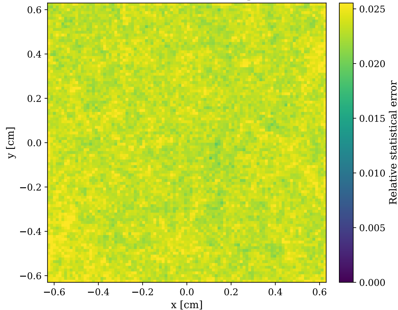
Flux Relative Error Map
