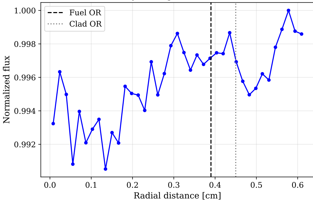
Azimuthally-Averaged Radial Flux Profile
