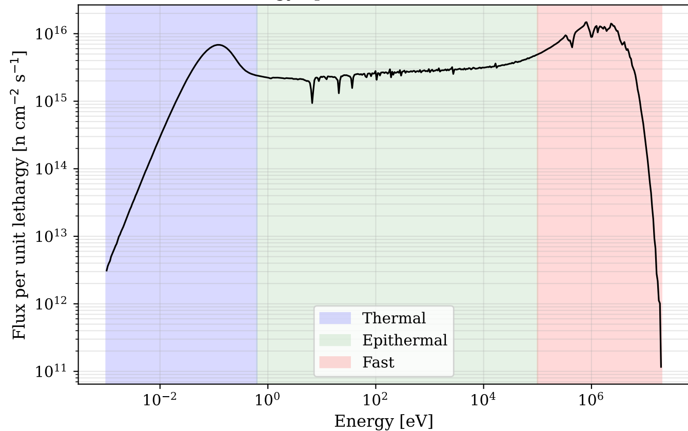
Neutron Energy Spectrum (Idealized PWR Pin Cell)
