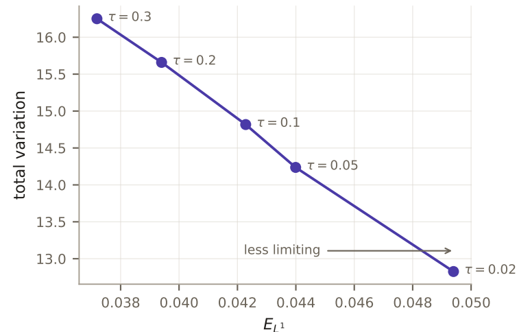
Shu-Osher threshold trade-off (1D GNN, K = 300 )
