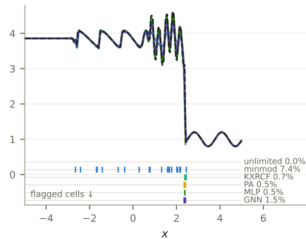
Shu-Osher threshold trade-off (1D GNN, K = 300 )
