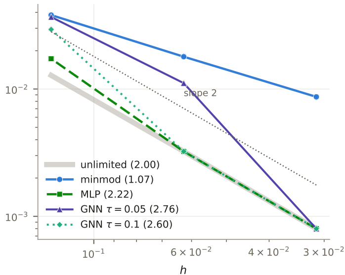
2D smooth advection, p = 1 (legend: fitted L^2 slope)
