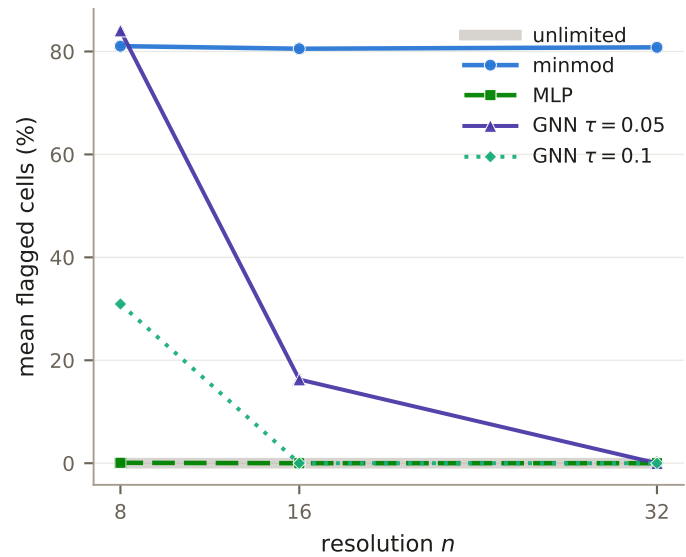
2D activity on a smooth field (ideal: 0%)
