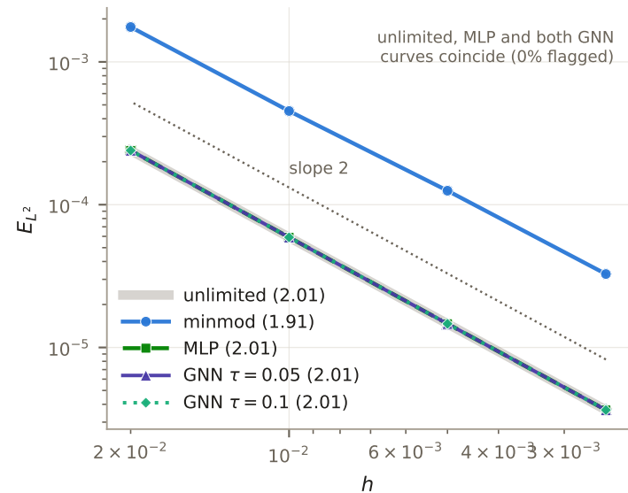
1D smooth advection, p = 1 (legend: fitted L^2 slope)
