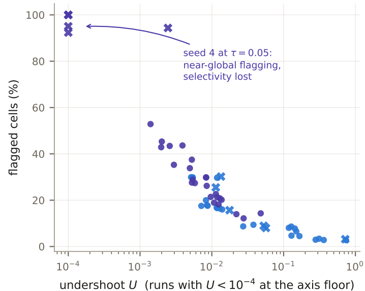
Per-run Pareto front (30 runs per \tau )
