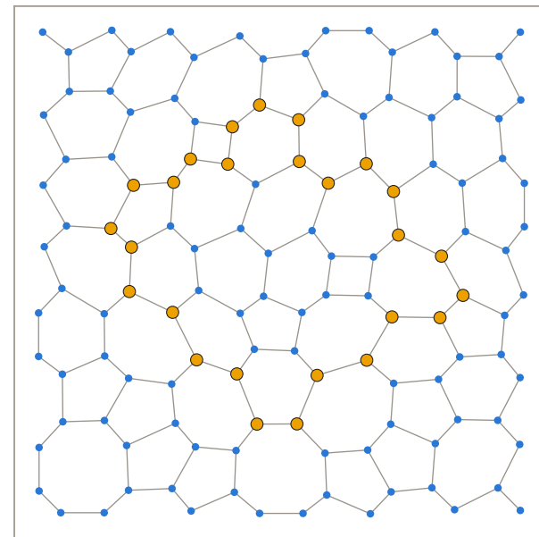
(f) face-adjacency graph
