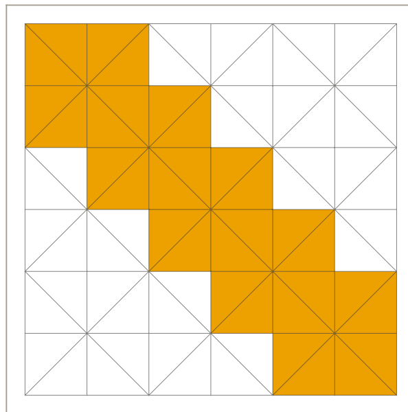
(e) intersected-cell labels
