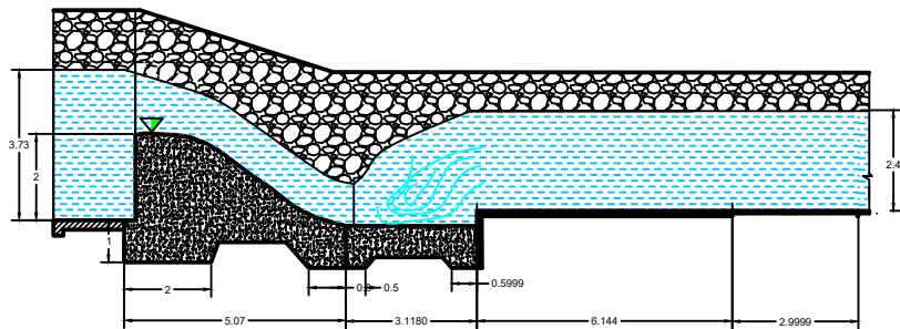
B-B Section
