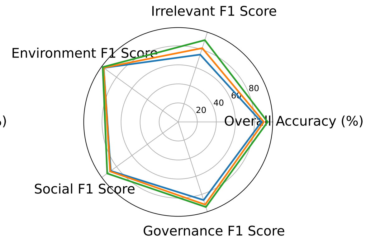
DistilBERT-base-multilingual
