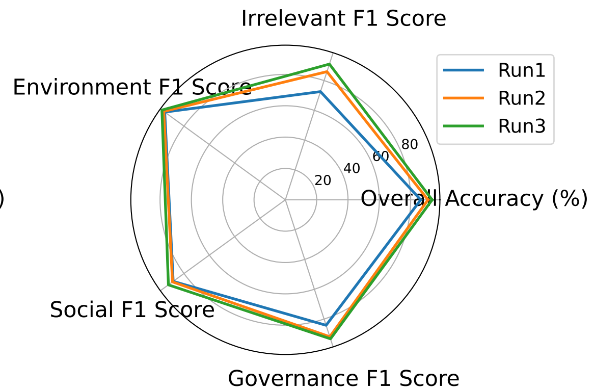
PhoBert
