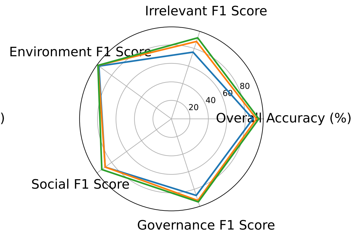
Vi-Electra
