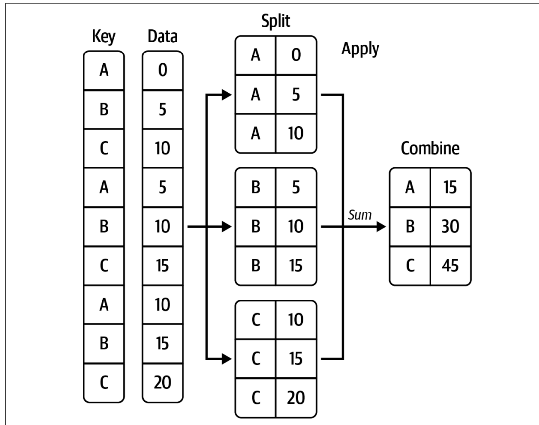
Figure 10-1. Illustration of a group aggregation
