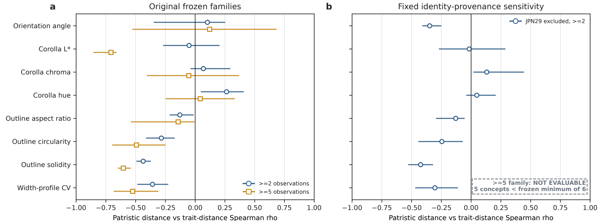
Figure S2. Continuous state-structure estimates and leave-one-out ranges
