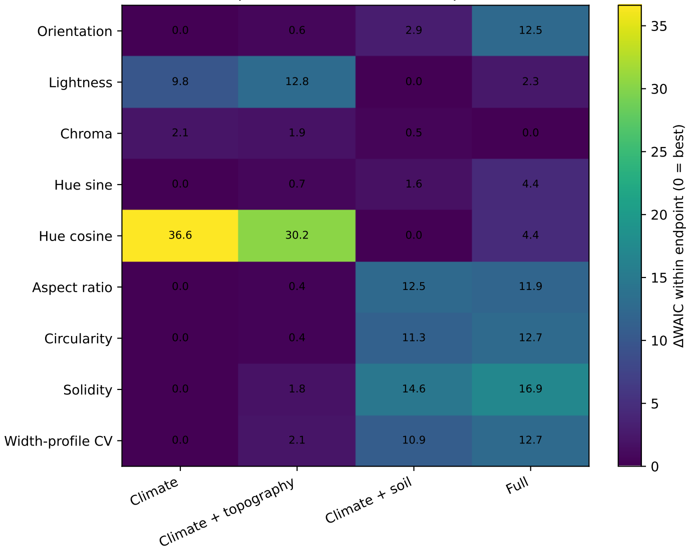
Grouped SPDE-INLA model comparison
