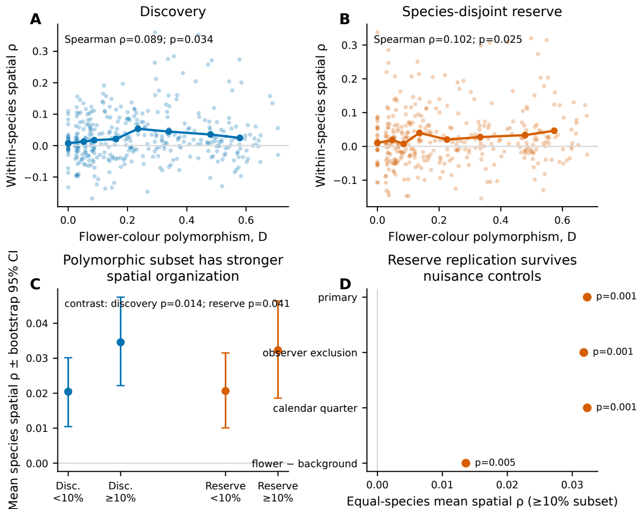
Figure 2 | Greater polymorphism predicts stronger within-species geographic organization
