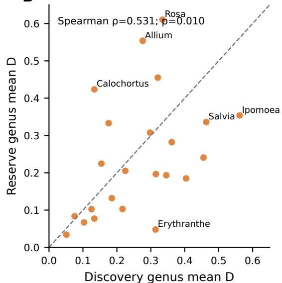
Figure 4 | Genus-level structure is a secondary, qualified result
